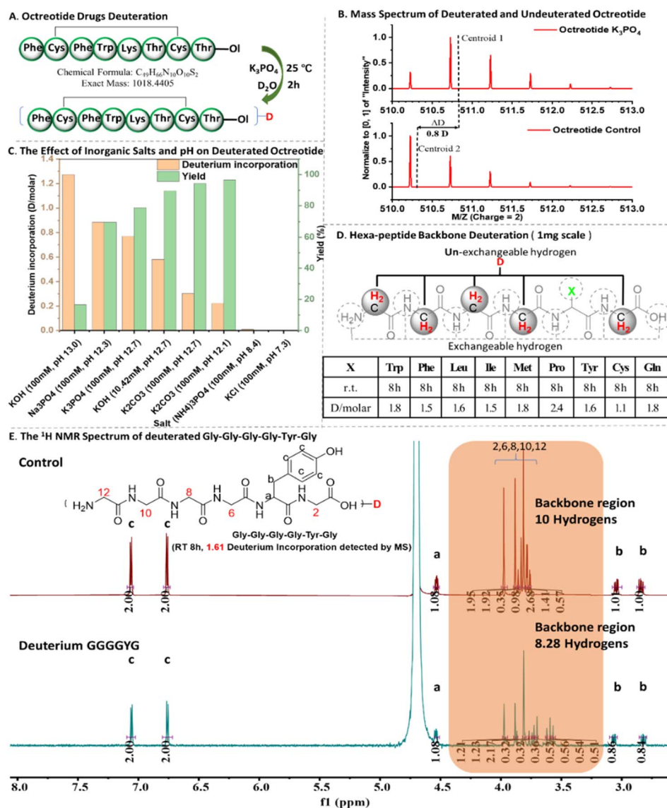
Fig. 2 The illustration of peptide deuteriation. (A) Octreotide deuteriation; (B) mass spectrum of deuterated and un-deuterated octreotide; (C) the effect of inorganic salts and pH value on octreotide deuteriation; (D) hexa-peptide backbone deuteriation (1 mg scale); (E) the comparison of ^1\text{H} NMR spectrum of deuterated Gly-Gly-Gly-Gly-Tyr-Gly (GGGGYG) and un-deuterated GGGGYG (other hexa-peptides ^1\text{H} NMR spectrums are provided in ESI.†).
